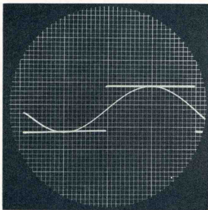
Figure 3. A 600-cycle sinewave and a 60-cycle square wave calibrating signal of equal amplitude shown superimposed for purposes of illustration. In actual practice the substitution method of calibration would be used if a dual-beam cathode-ray oscillograph were not employed
