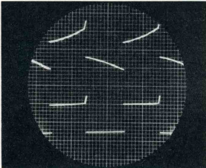
Figure 6. The same low-frequency square-type wave applied to both channels of the Type 322. Upper waveform shows a-c coupling and lower d-c coupling. Tilt in the tops of the upper waveform is caused by time constants in the a-c coupling circuit
