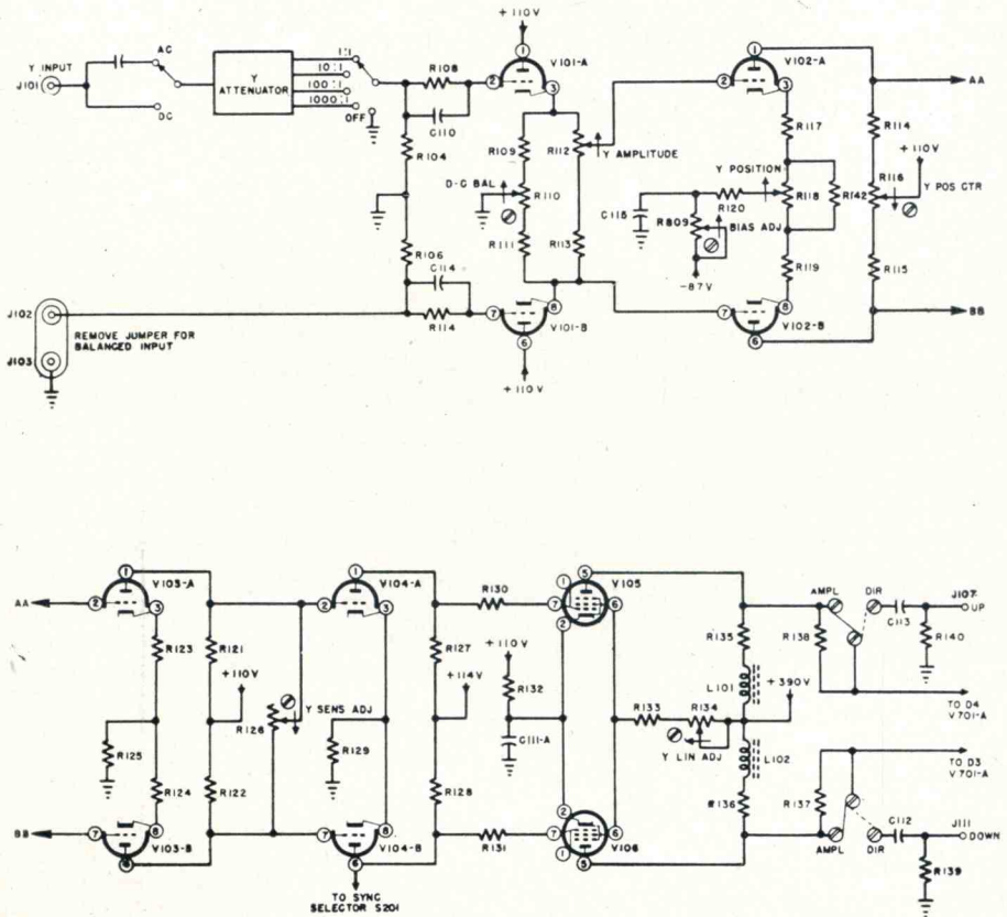
Figure 2. Y-axis amplifier circuit
