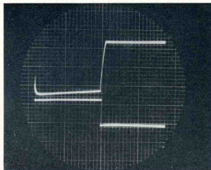
Figure 5. Input (lower trace) and output (upper trace) of an amplifier circuit using the common sweep of the new Type 322. The frequency is 1 KC. Note how the loss in rise time may be conveniently measured
