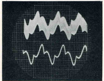
Figure 7. Complex waveform from a balanced output is displayed with balanced input (upper trace) and with single-ended input (lower trace)
