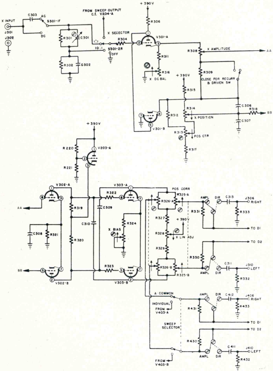
Figure 4. X-axis amplifier circuit, simplified schematic
