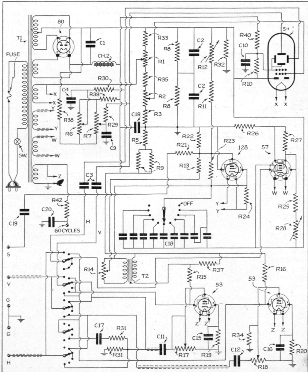
Fig. 29A. Schematic of Model 148 Dumont 3" Oscillograph
