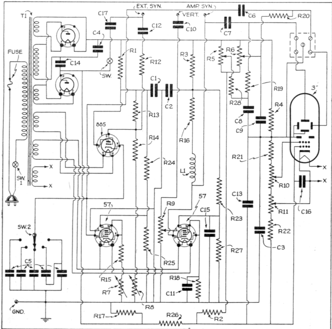
Fig. 50. Schematic of Model 154 Dumont 3" Oscillograph.
