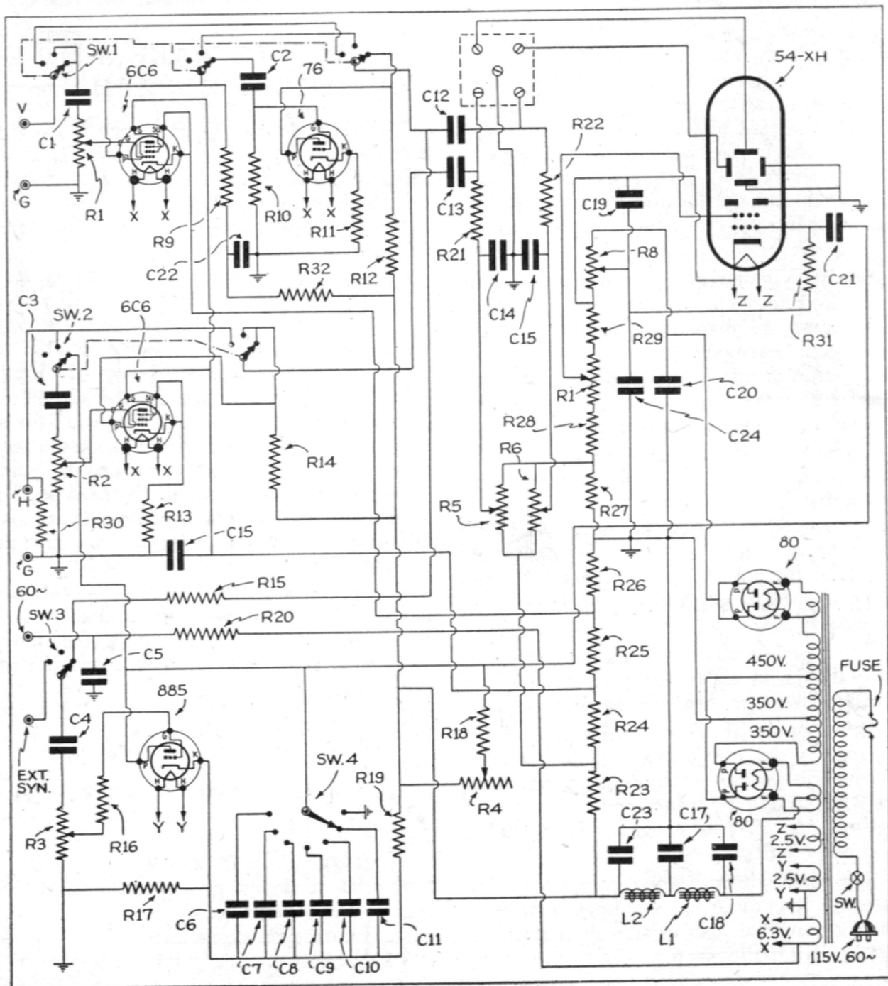
Fig. 51A. Schematic of Model 168 Dumont 5" Oscillograph
