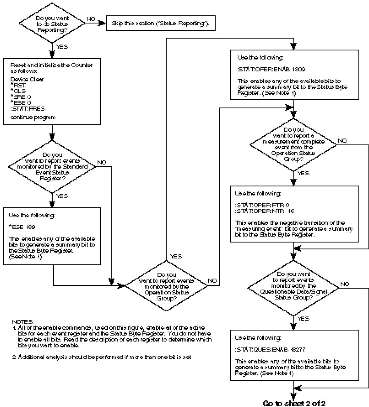
Figure 3-10. Status Reporting Flowchart (1 of 2)
