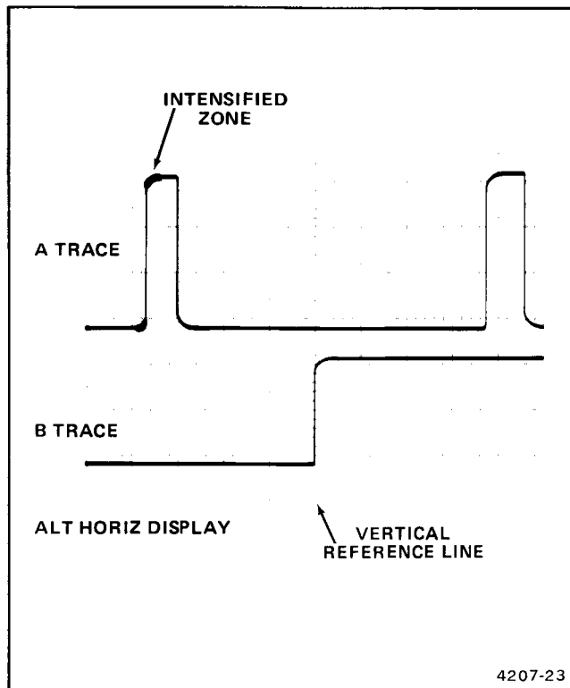
Figure 4-13. Time difference between repetitive pulses.
