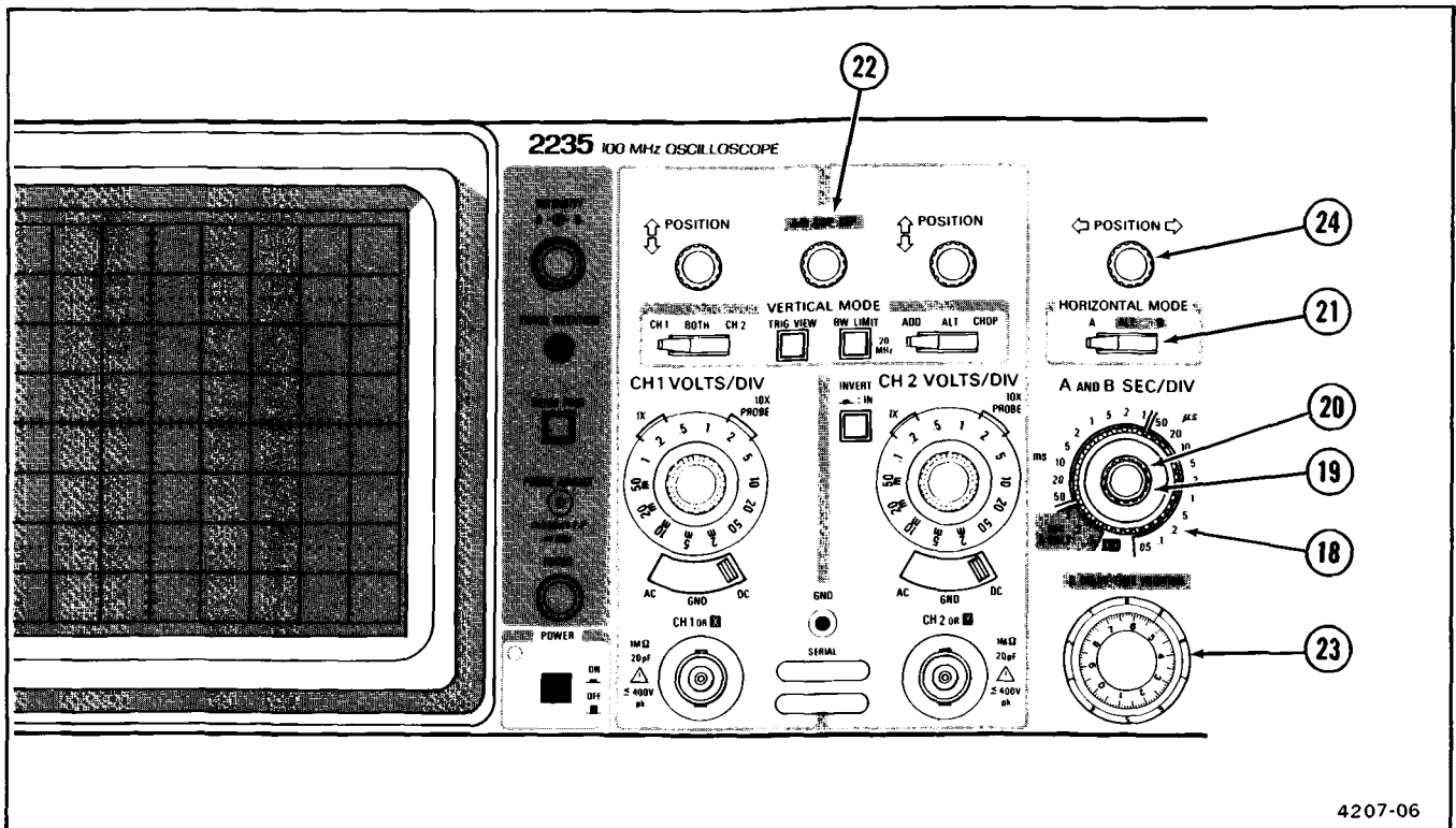
Figure 2-5. Horizontal controls.
