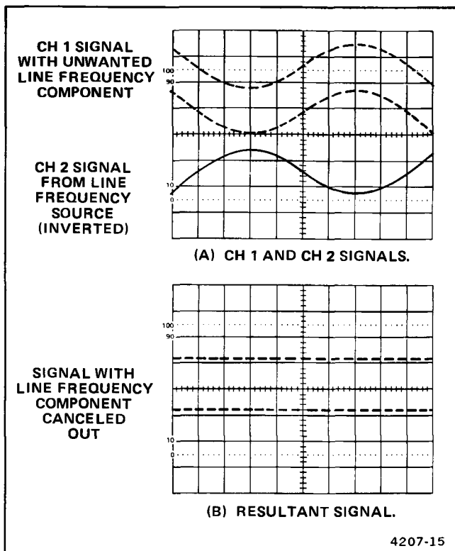
Figure 4-5. Common-mode rejection.
