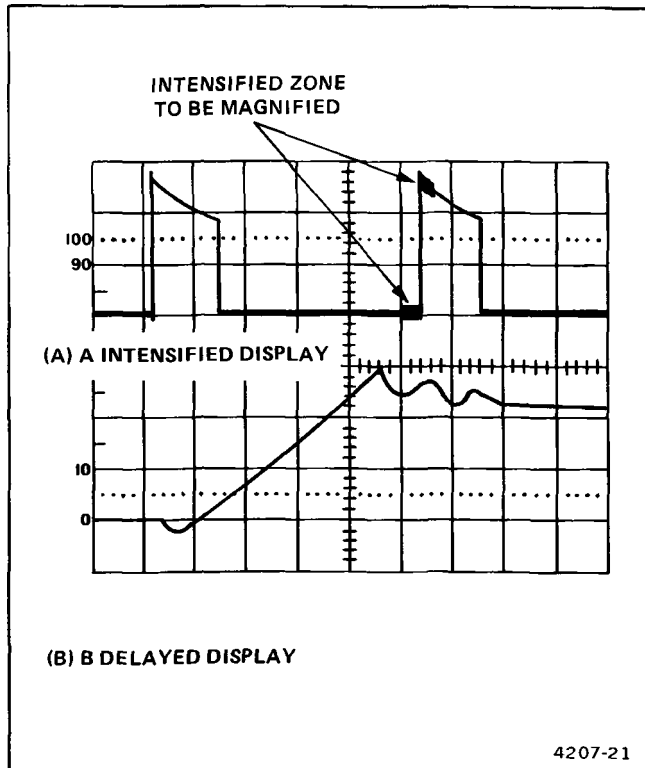
Figure 4-11. Delayed-sweep magnification.
