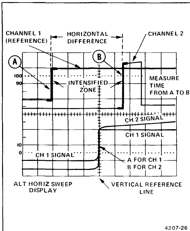
Figure 4-16. Time difference between two time-related pulses, differential time method.
