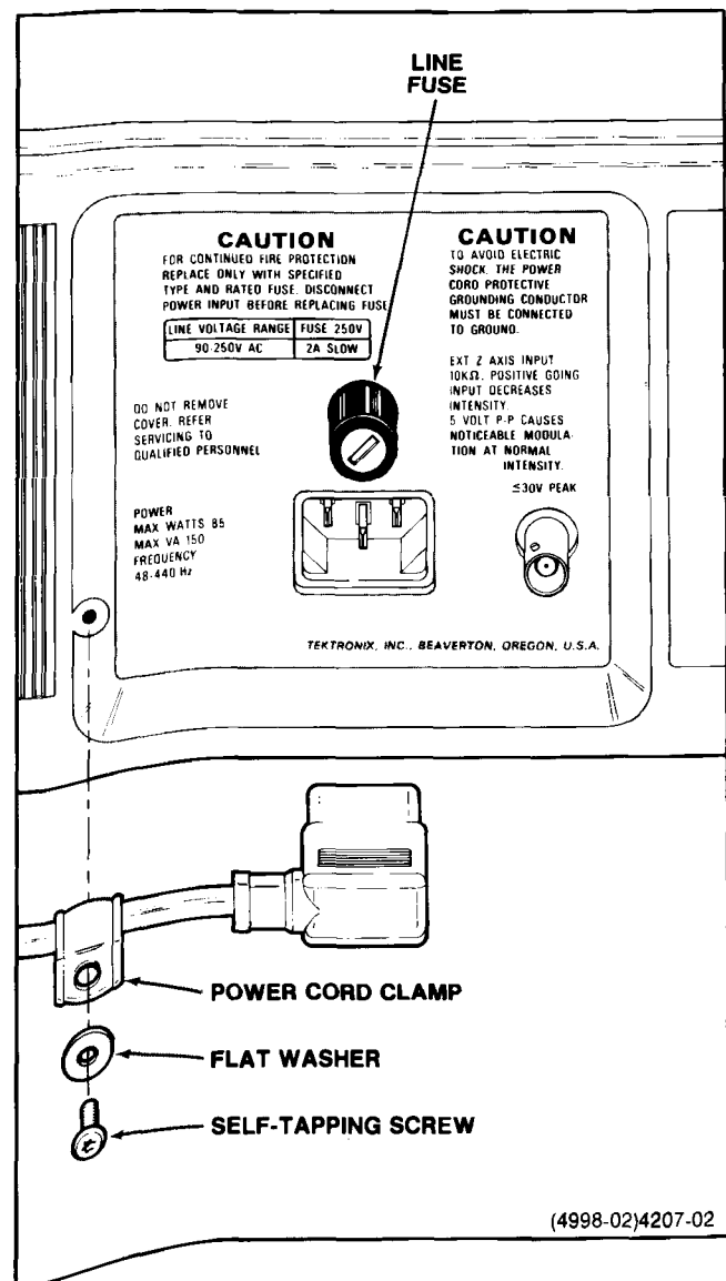
Figure 2-1. Power cord clamp and line fuse.
