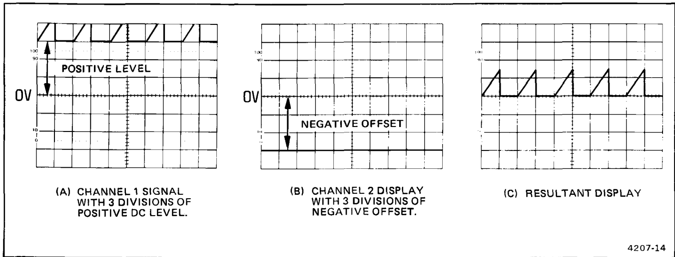
Figure 4-4. Algebraic addition.
