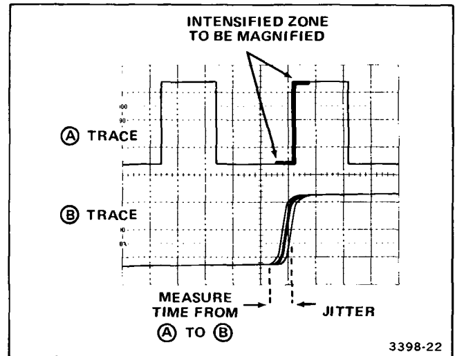
Figure 4-12. Pulse jitter.
