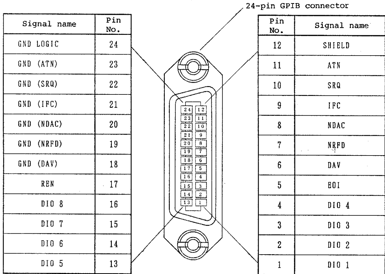
Figure 3-2 GPIB connector pin layout
