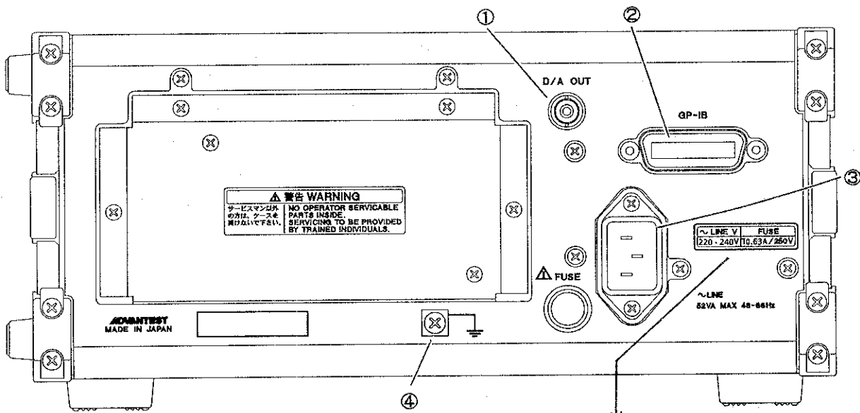
Rear panel
