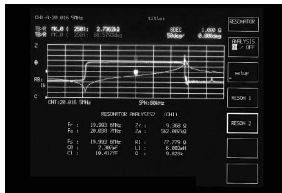
Resonator 2 measurement
