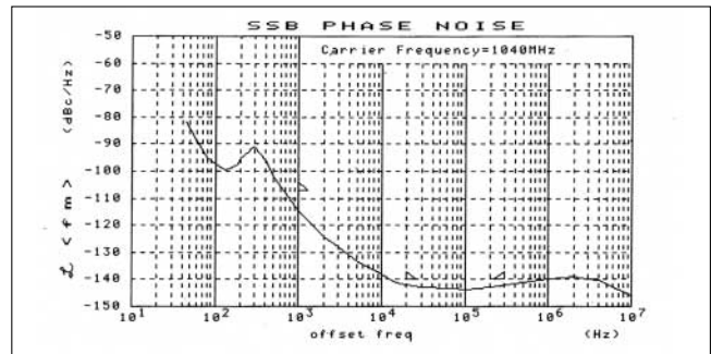
Figure 1. SSB Phase Noise
