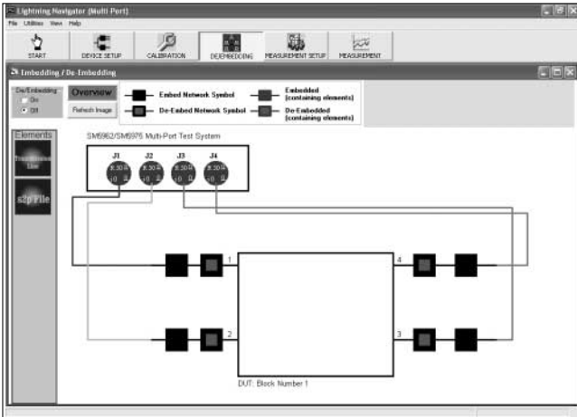
Embedding/De-Embedding
