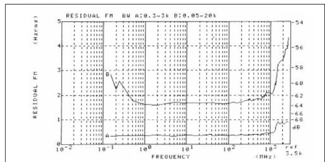
Figure 2. Residual FM
