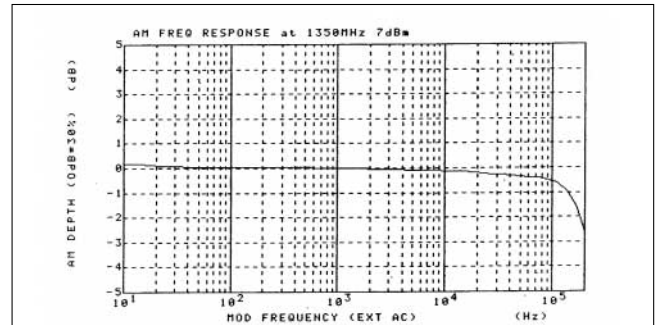
Figure 4. AM Modulation Frequency Characteristics
