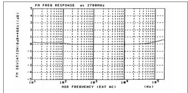
Figure 5. FM Modulation Frequency Characteristics
