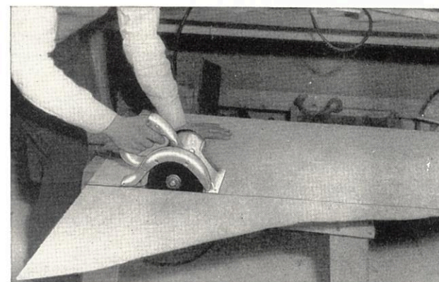
↑ Cutting transite with Abrasive Disc. This accessory also handles slate, tile, marble, ceramics, etc.
