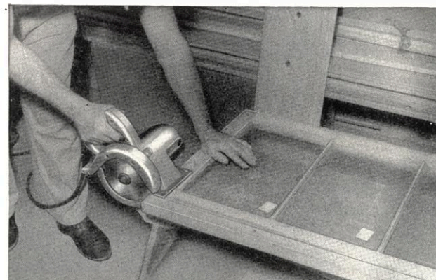
↑ Making a fast, clean cut in trimming stock size windows, doors and screens to fit.
