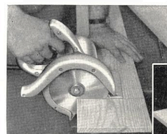
Motor housing makes convenient extra hand grip when desired.
