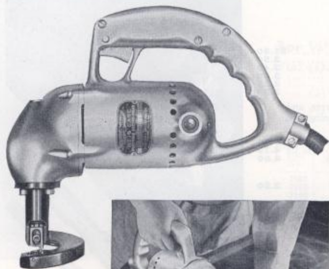
16 GAGE PORTO-SHEAR
