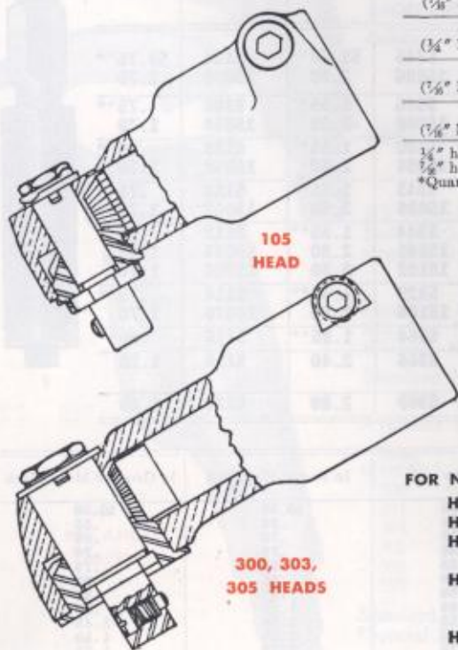
RIGHT-ANGLE HEADS
