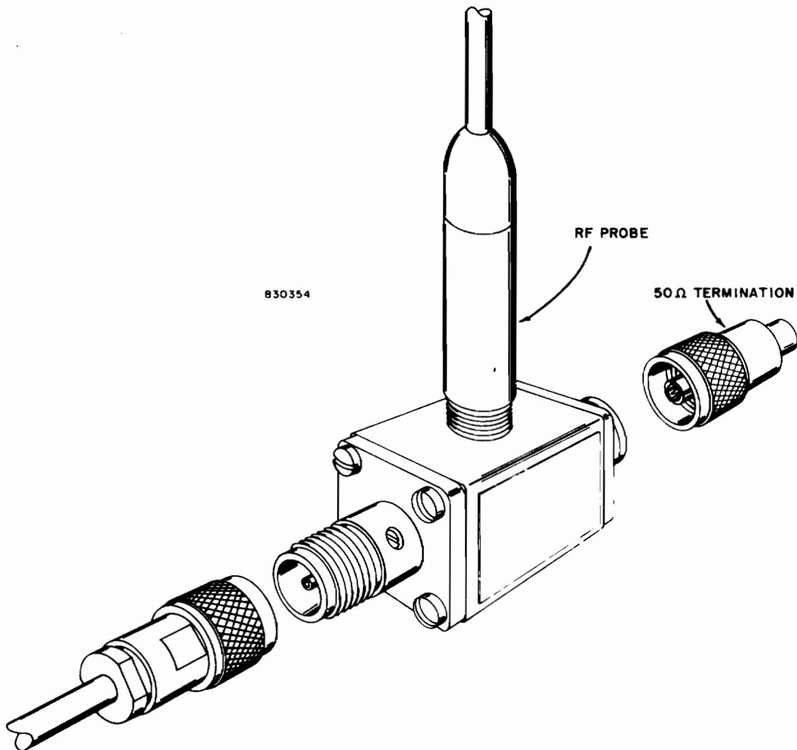
Figure 2-1. Assembly of Type N Tee Adapter
