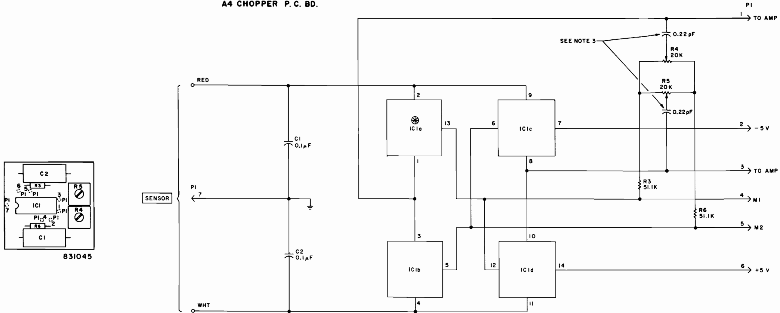
Parts-Location Diagram (B831045D)
