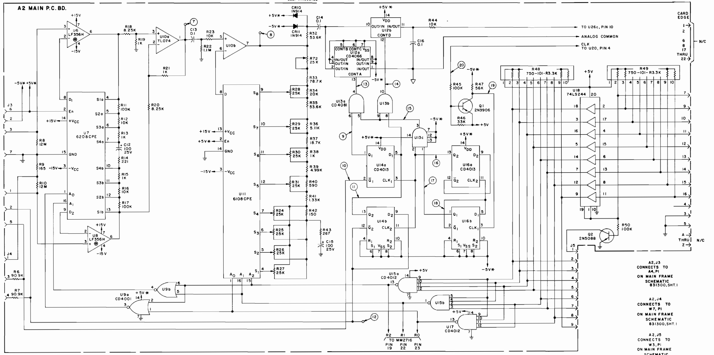
SCHMATIC MAIN P.C. BOARD E831300 E SHT.2b of 2
