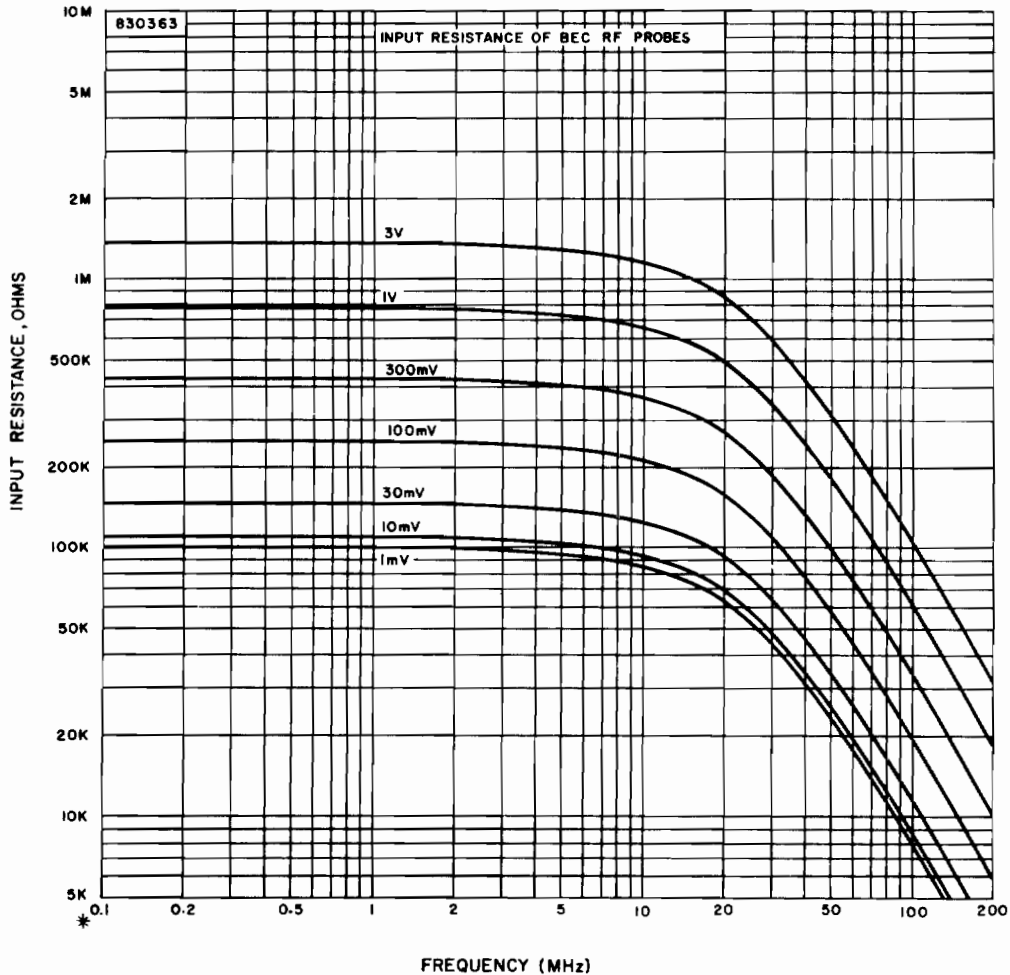
Figure 1-1. Input Resistance of Model 952001-02A R.F. Probe as a Function of Input Level and Frequency
