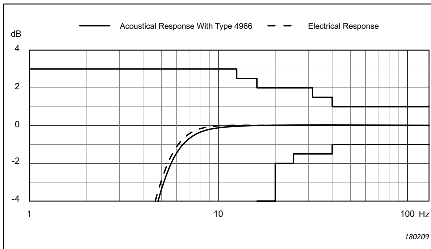
Fig. 4.2 Typical low-frequency responses
