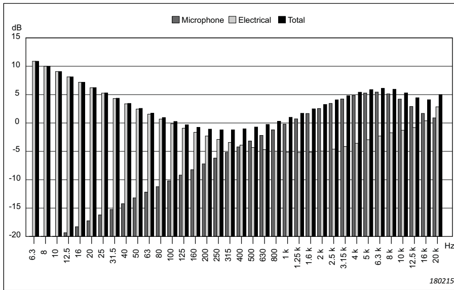
Fig. 4.14 Typical self-generated noise, 1/3 octave band
