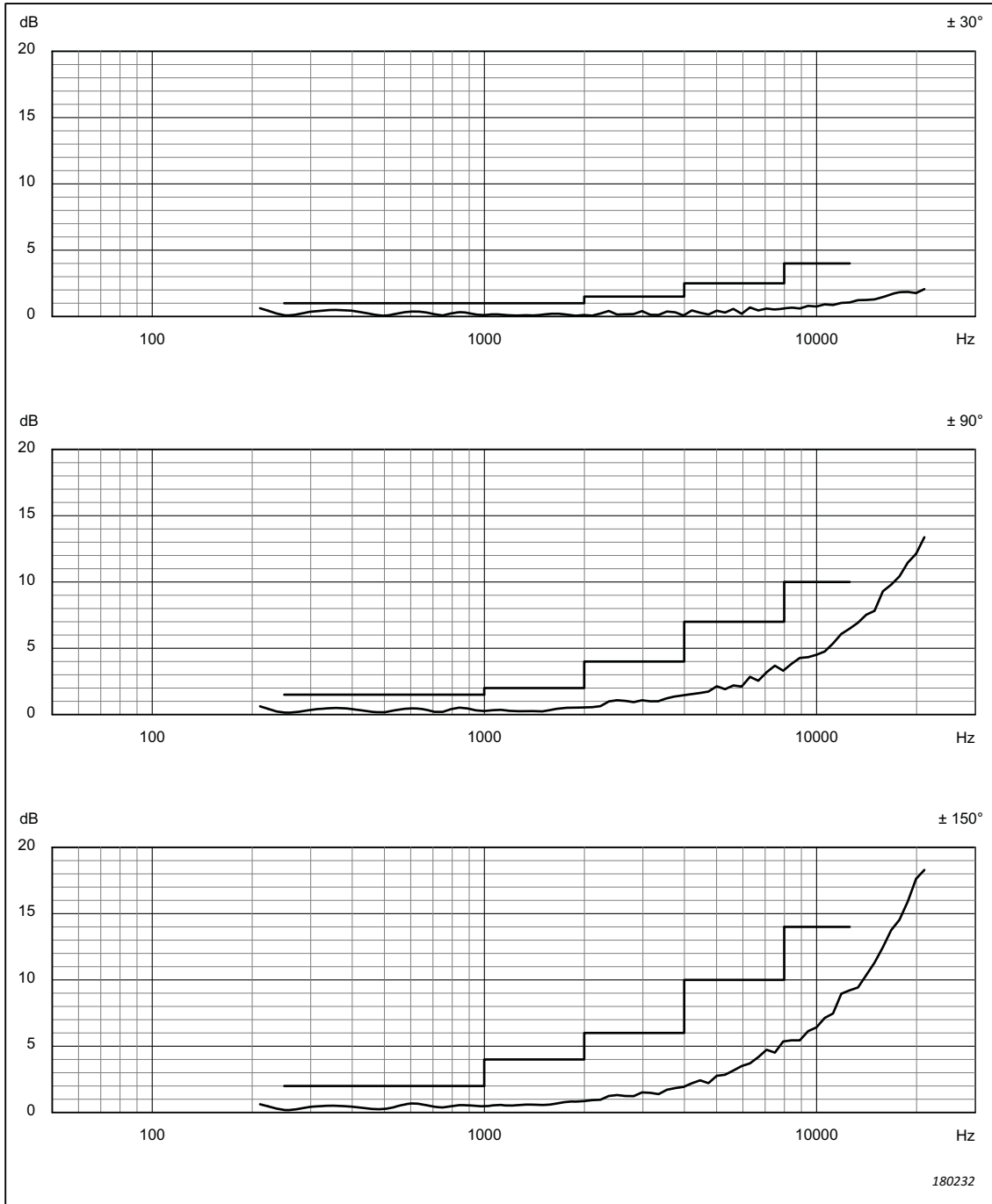
Fig. 4.9 Sensitivity variations for the sound level meter at sound incidence angles within \pm\theta^\circ from the reference direction. Corresponds to Table A.13
