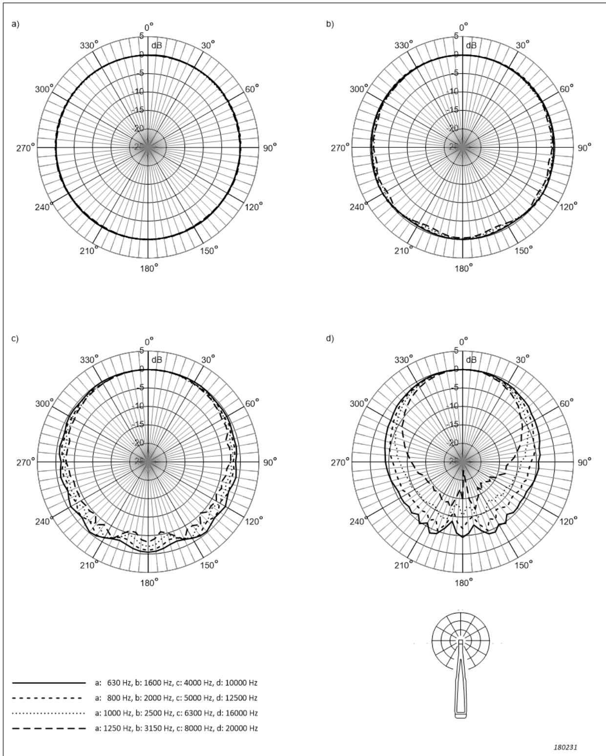
Fig. 4.8 Directional response for the sound level meter measured in a plane perpendicular to the display and along the microphone axis. Corresponds to Table A.10 to Table A.12
