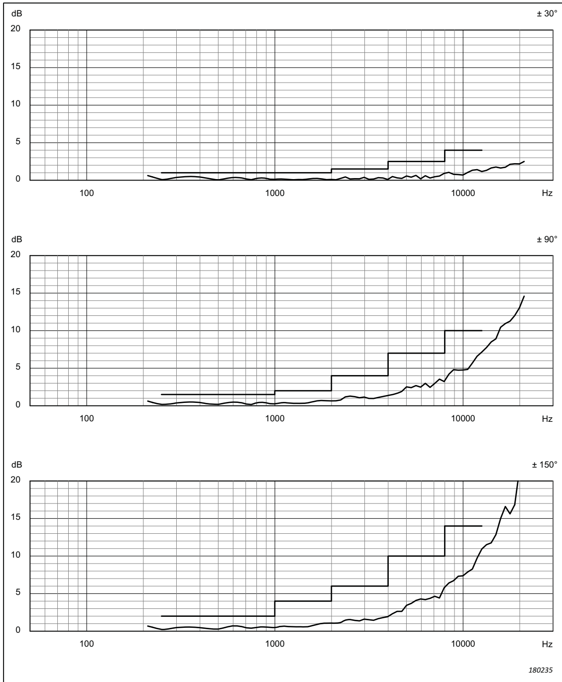
Fig. 4.12 Sensitivity variations of the sound level meter with Windscreen UA-1650, at sound incidence angles within \pm\theta^\circ from the reference direction. Corresponds to Table A.23
