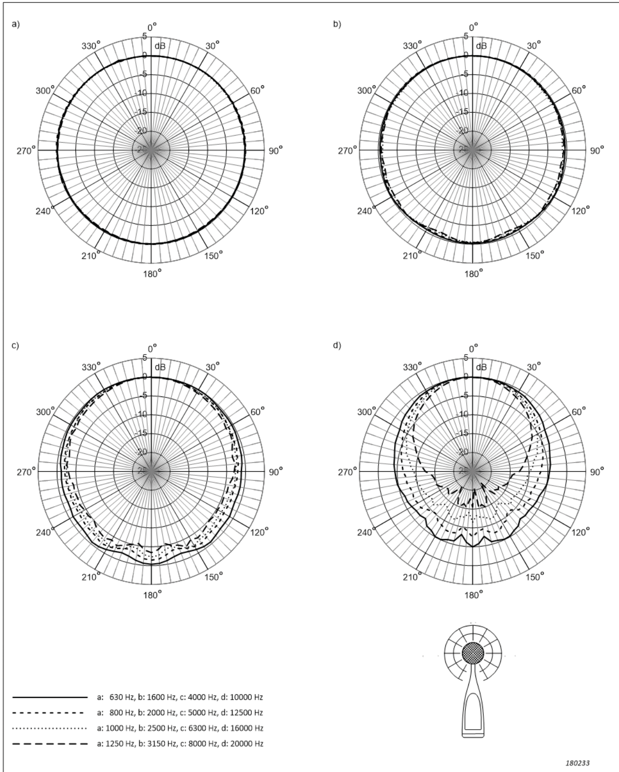
Fig. 4.10 Directional response for the sound level meter with Windscreen UA-1650, measured in a plane parallel to the display and along the microphone axis. Corresponds to Table A.17 to Table A.19
