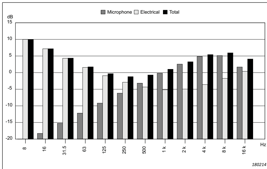
Fig. 4.13 Typical self-generated noise, 1/1-octave band
