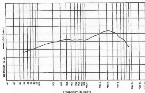
Figure 3 - Frequency Response
