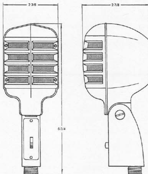
Figure 1 - Dimensions
