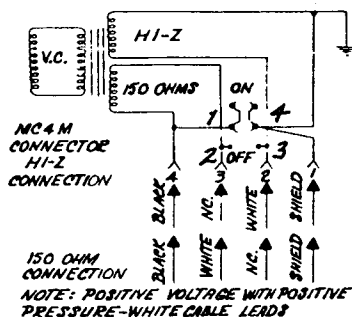
Fig. 5 — Wiring Diagram
