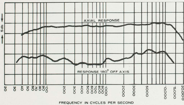
Figure 2 - 666 Frequency Response
