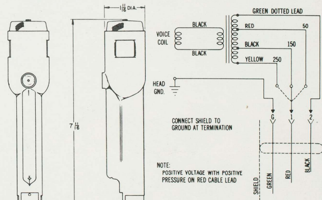
Figure 5 - Wiring Diagram
