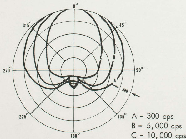
Figure 3 - Polar Pattern
