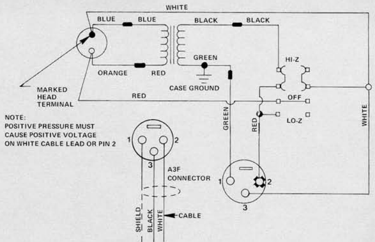
FIGURE 4 – Wiring Diagram
