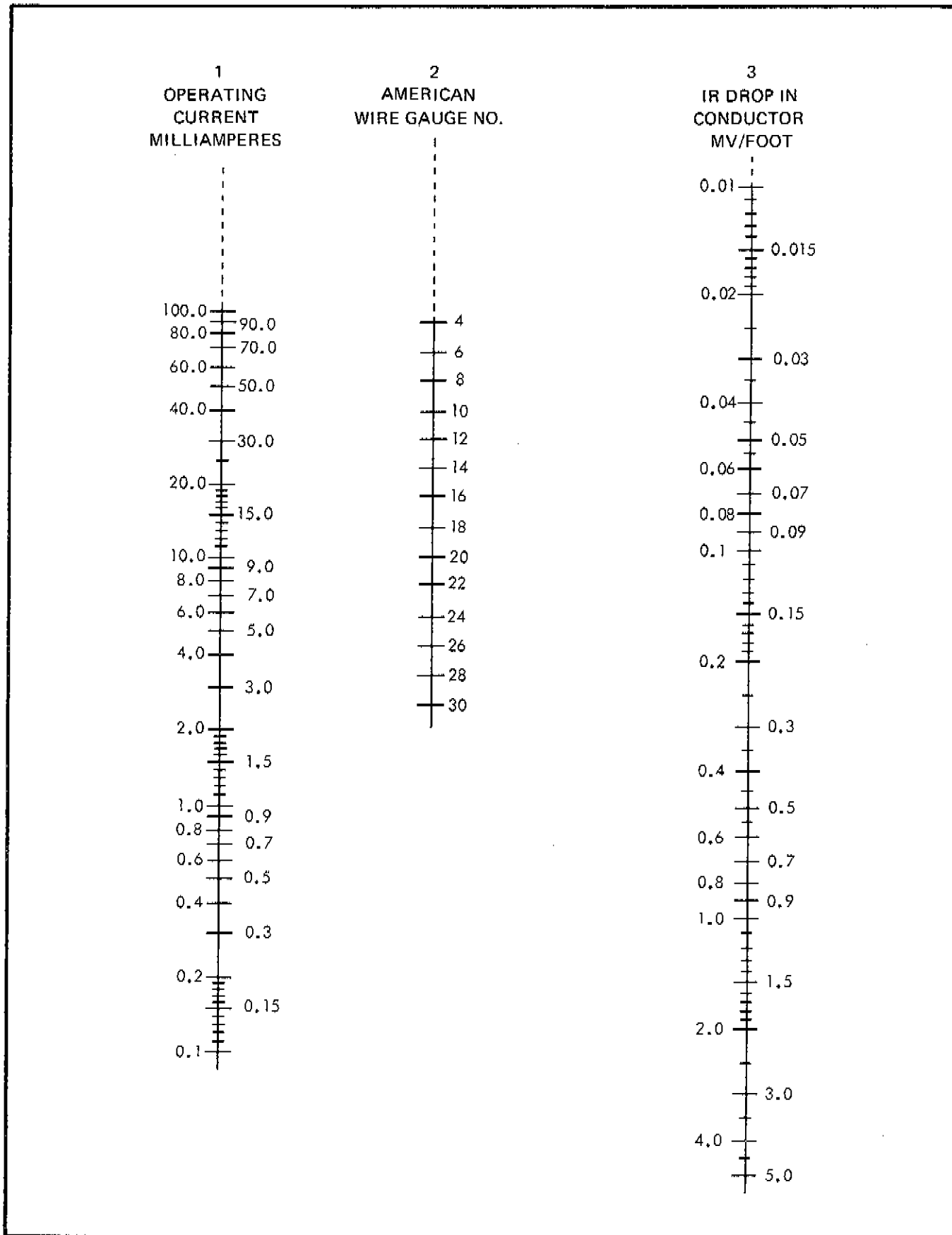
Figure 2-2. NOMOGRAPH OF VOLTAGE DROP IN LOAD WIRES
