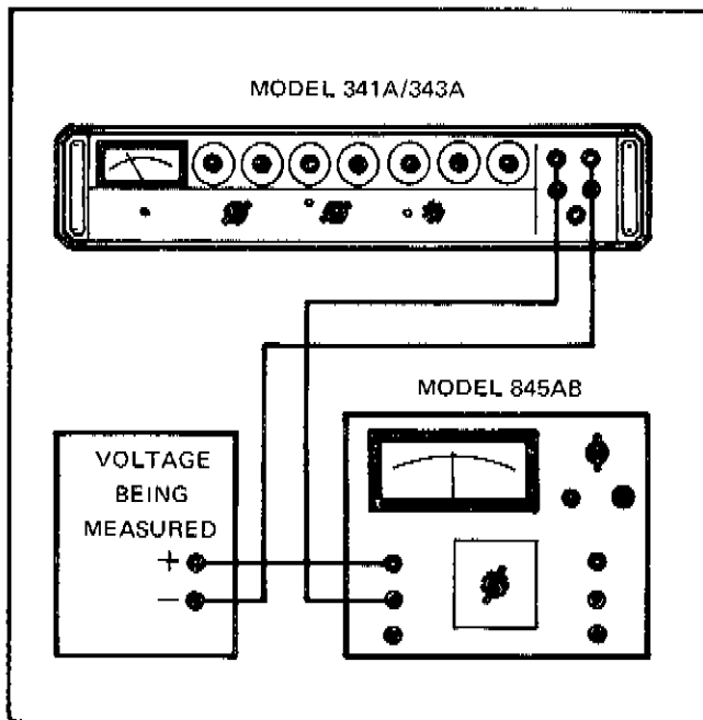
Figure 2-3. DIFFERENTIAL VOLTMETER
