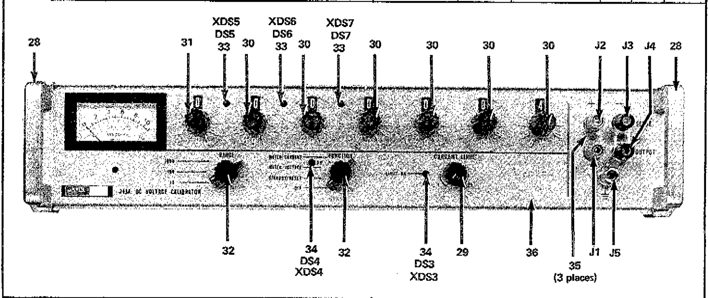
Figure 5-9. FRONT PANEL ASSEMBLY (343A)
