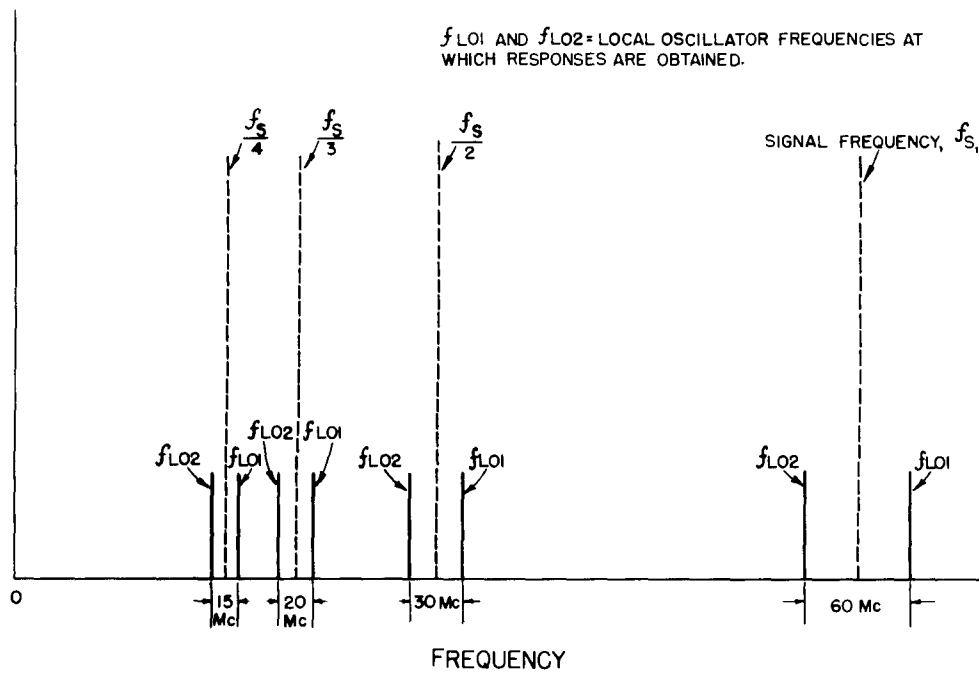
Figure 12. Chart showing local oscillator frequencies at which responses will be produced with various local oscillator harmonics.
