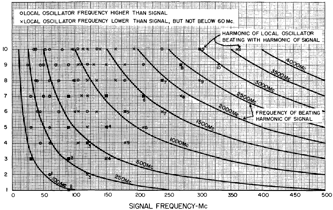
Figure 14. Signal frequencies at which overlapping harmonic responses can be obtained as a result of harmonics of the signal frequency beating with different harmonics of the local-oscillator frequency and producing 30-Mc difference frequencies.
