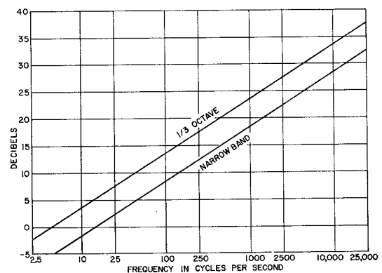
Figure 12. Decibels to Be Subtracted from Type 1564-A Reading to Obtain Spectral-Density Level.
