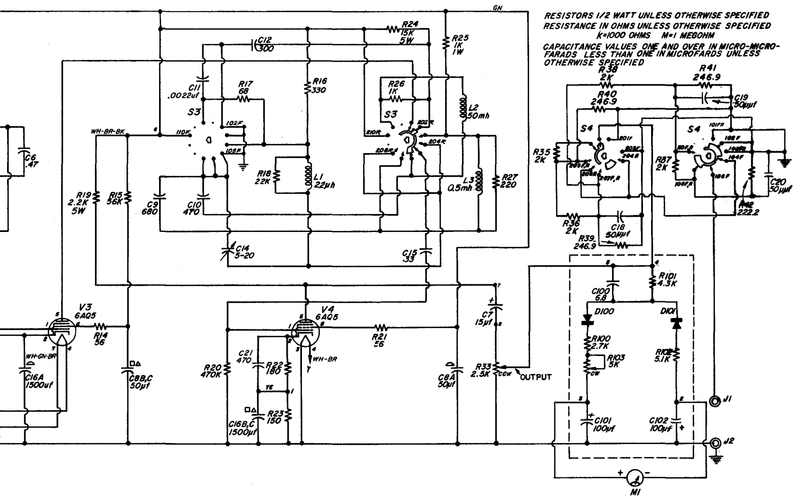
Figure 12. Schematic Wiring Diagram.
