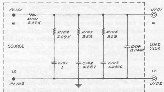
Figure 10. Schematic diagram of the Pink-Noise Filter.
