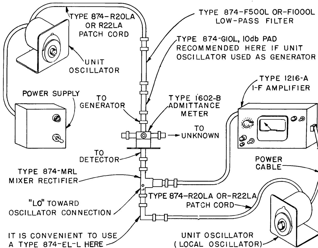
Figure 2c. Diagram of a measurement setup using a unit oscillator as a generator and the combination of a mixer rectifier, unit oscillator, and i-f amplifier as a detector.
