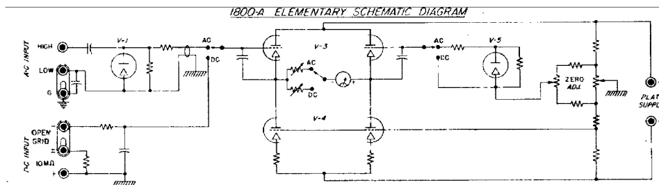
Figure 2. Schematic diagram of Type 1800-A Vacuum-Tube Voltmeter.
