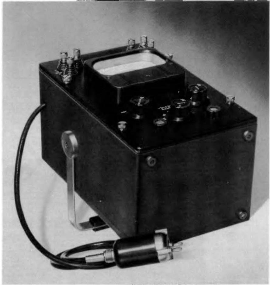
Figure 1. Panel view of the Type 1800-A Vacuum-Tube Voltmeter (left) with handle in vertical carrying position, and (right) with the handle locked in position for supporting instrument with inclined panel.
