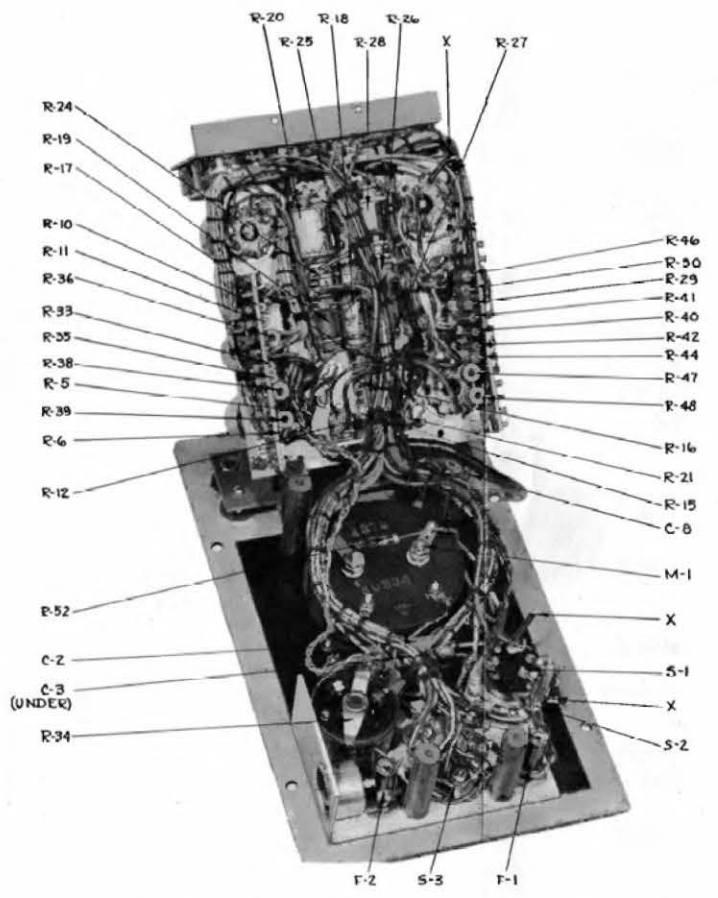
Figure 9. Interior view after subpanel has been laid back (see Section 14.2 of Service and Maintenance Notes).
