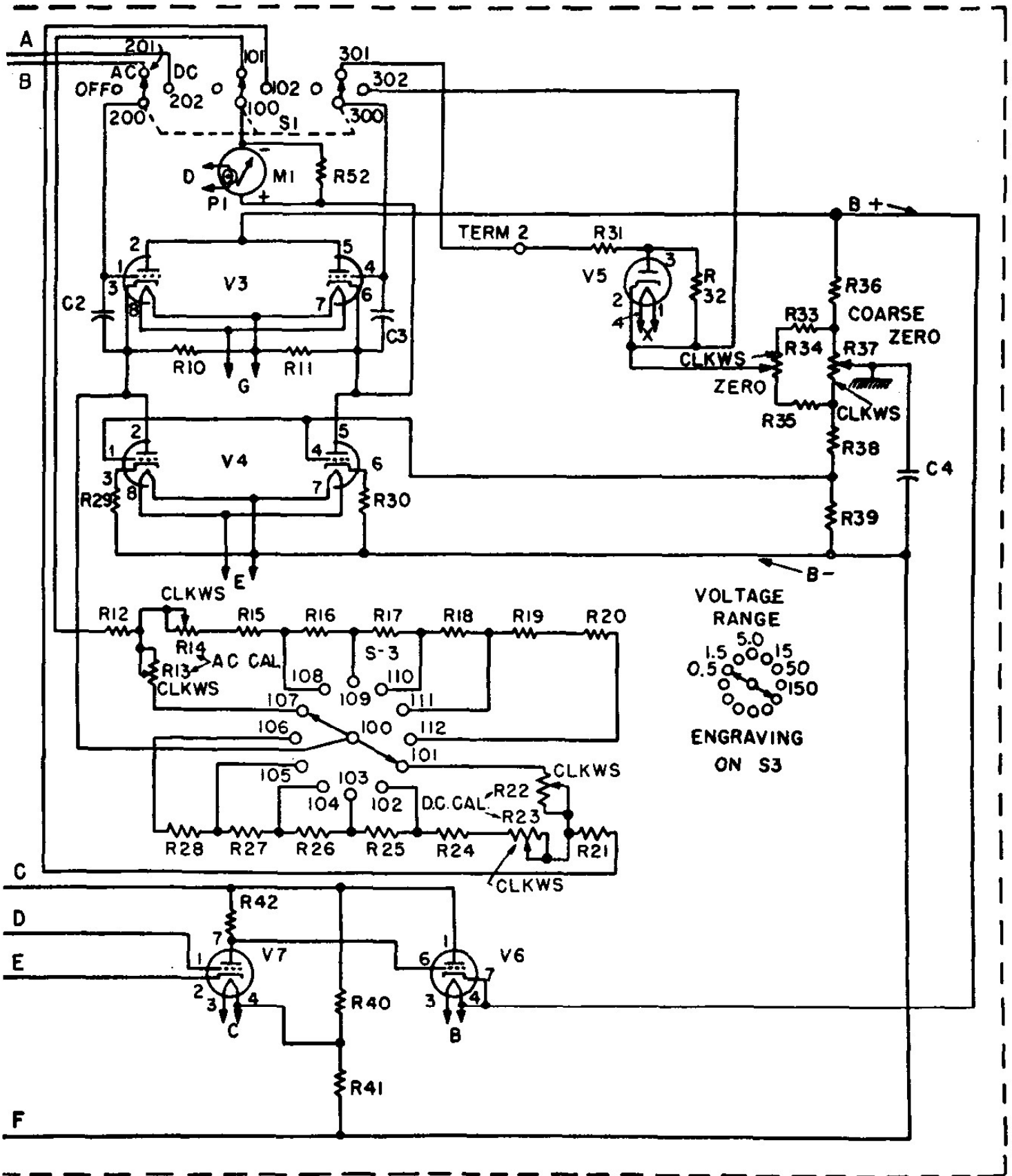
Model 1800A
