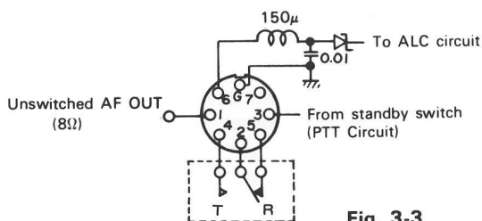
INTERNAL WIRING IN THE TS-130S(V)
