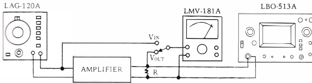
Fig. 2-1 Equipment and connections for measurements.
