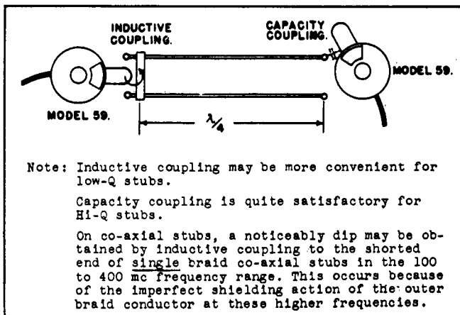
Figure 11 - COUPLING TO QUARTER-WAVE STUBS
