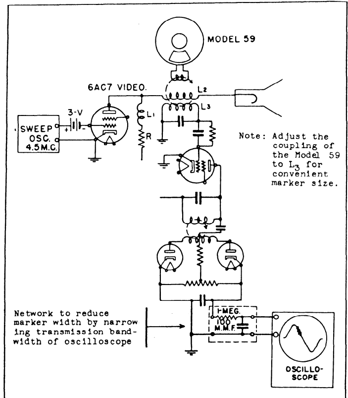
Figure 5 - USE OF MODEL 59 AS TRACE MARKER
