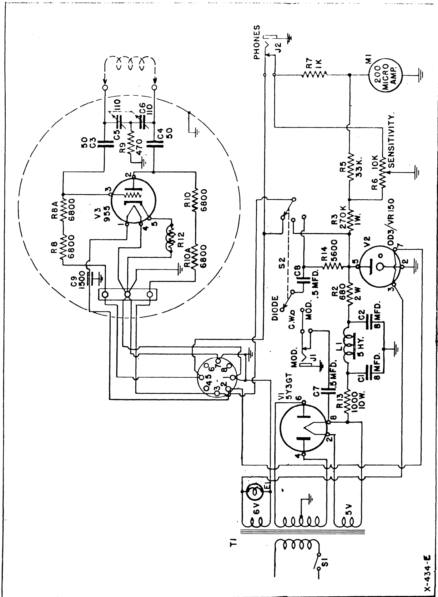
FIG. 18 - SCHEMATIC DIAGRAM.
