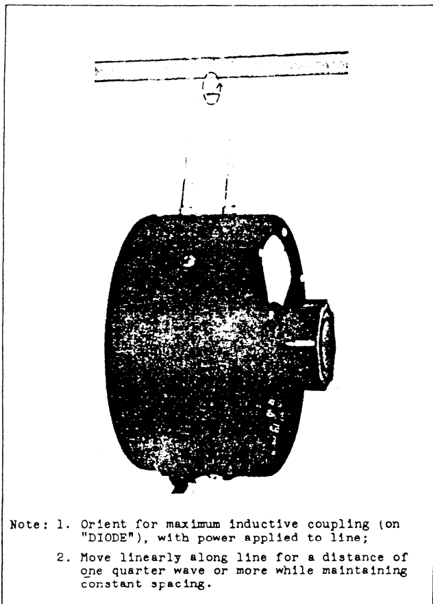
Figure 10 - CHECKING FOR STANDING WAVES ON TRANSMISSION LINES
