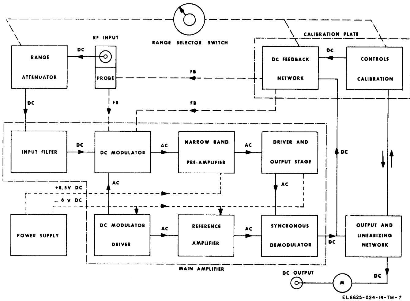
Figure 5-1. Block diagram.
