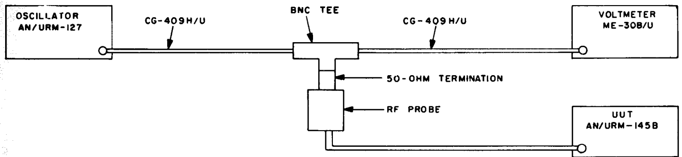
Figure 7-3. Voltage accuracy test setup.
