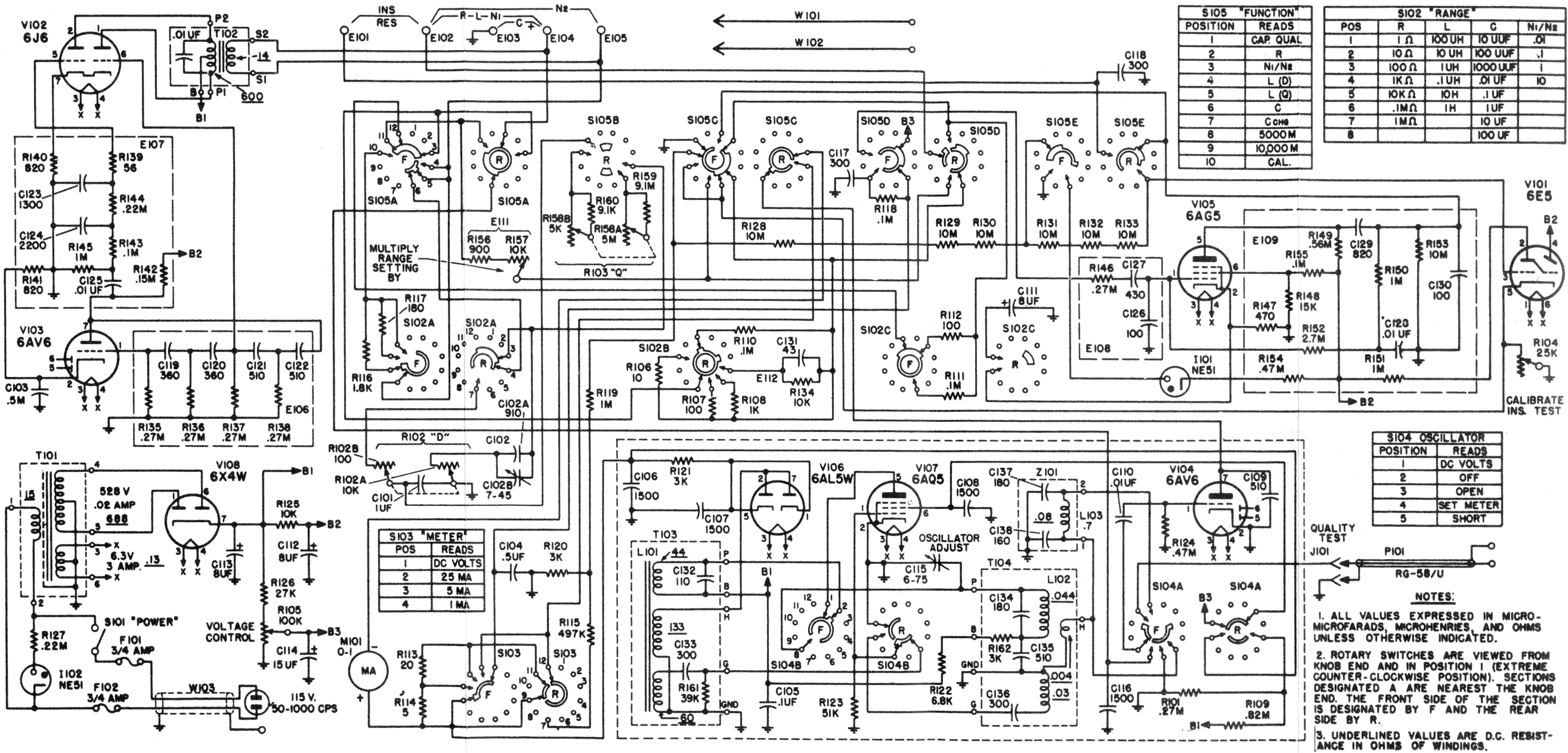
Figure 5-14. Bridge, ZM-11/U, Schematic Diagram
