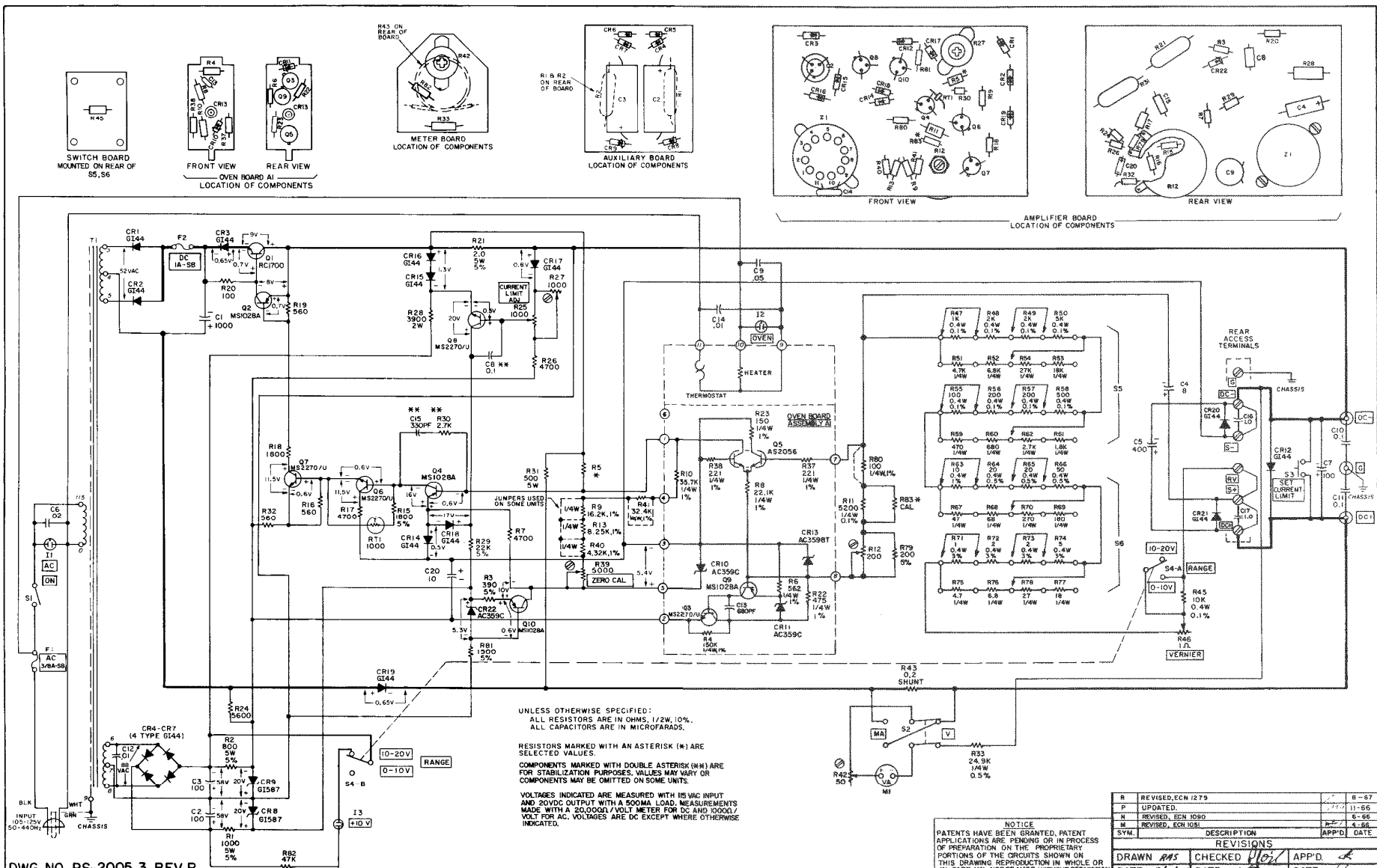
DWG. NO. PS-2005-3 REV R MODEL 2005 TRANSISTORIZED POWER SUPPLY
