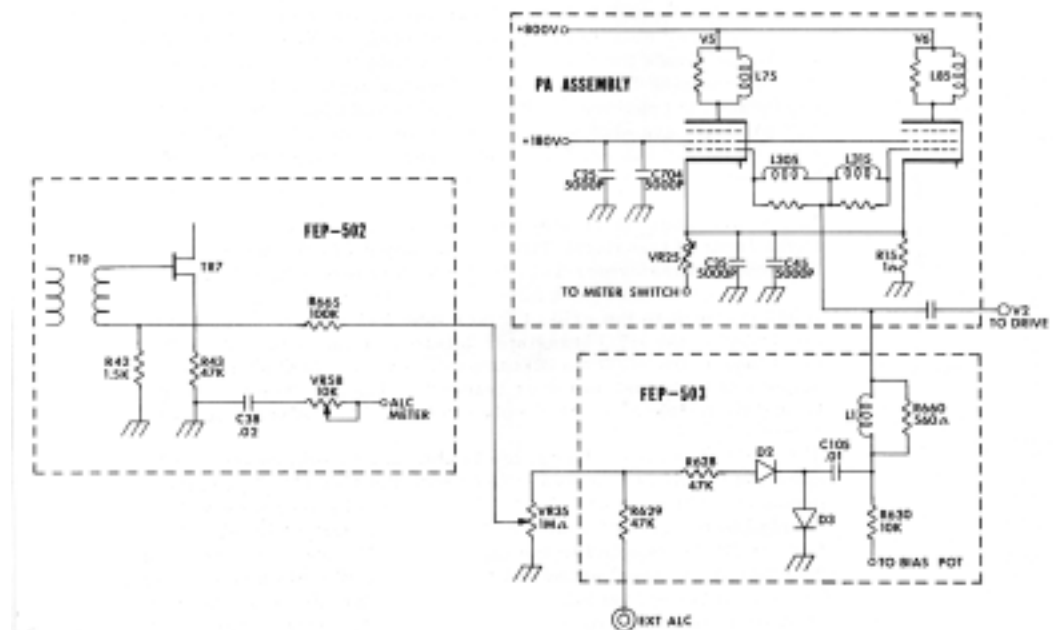
FIGURE 5.2 SIMPLIFIED ALC DIAGRAM
