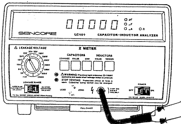
Fig. 7— Controls used for capacitor testing
