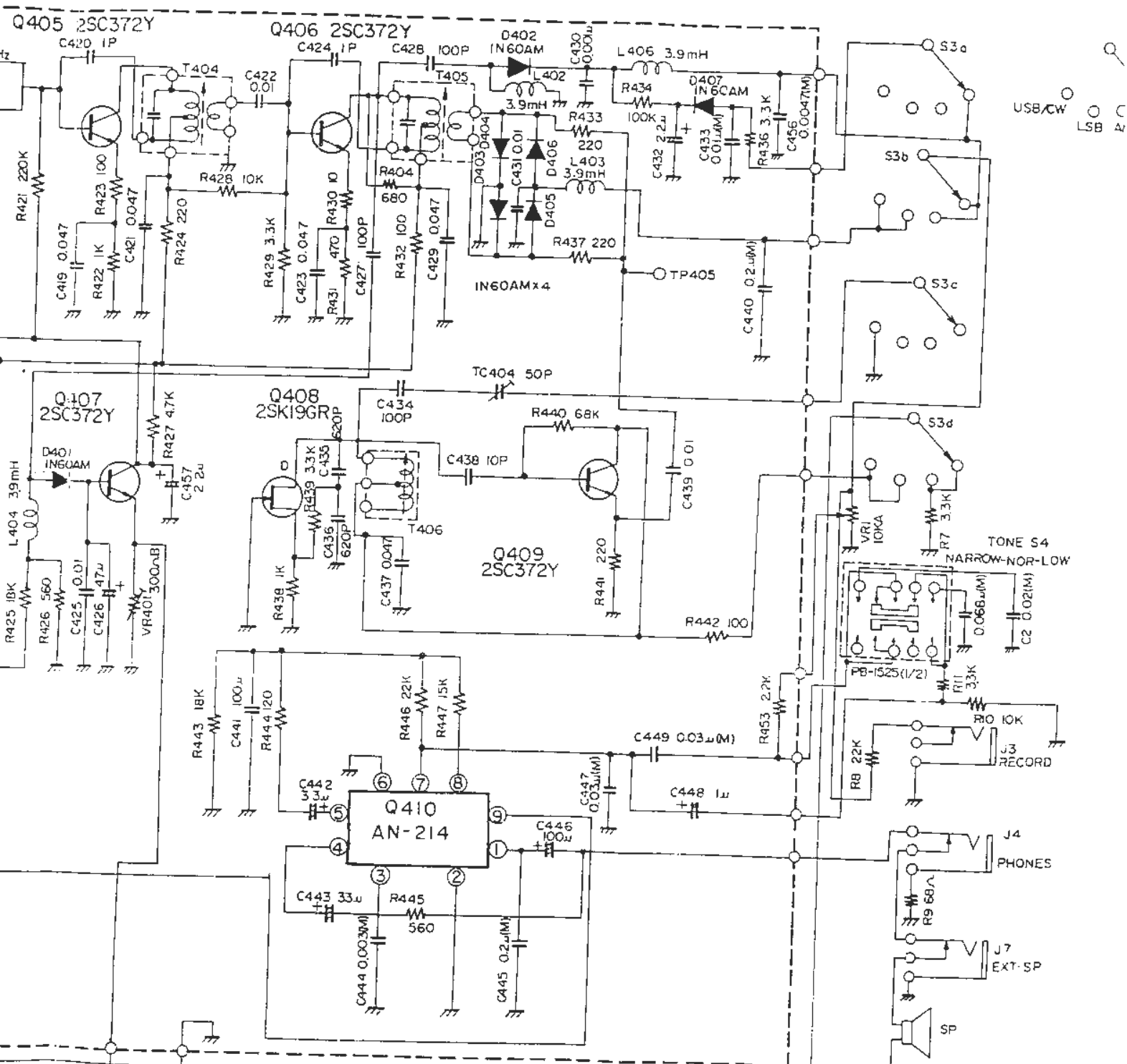
FRG-7 CIRCUIT DIAGRAM
